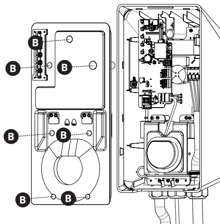
Tethered (Type 2 cable)
